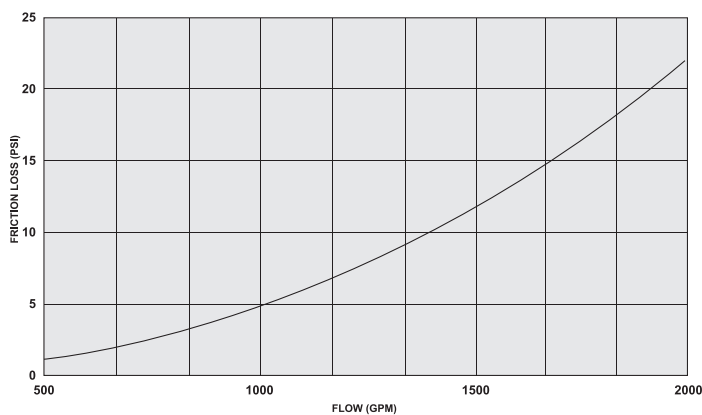
3671 CONQUEST MONITOR PERFORMANCE CHART
